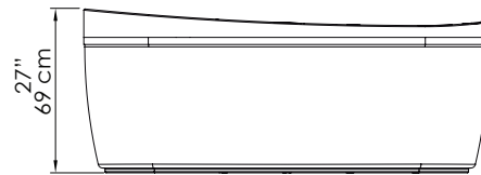
VISTA LATERAL / LATERAL VIEW
