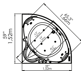
VISTA SUPERIOR / UPPER VIEW
