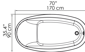
VISTA SUPERIOR / UPPER VIEW
